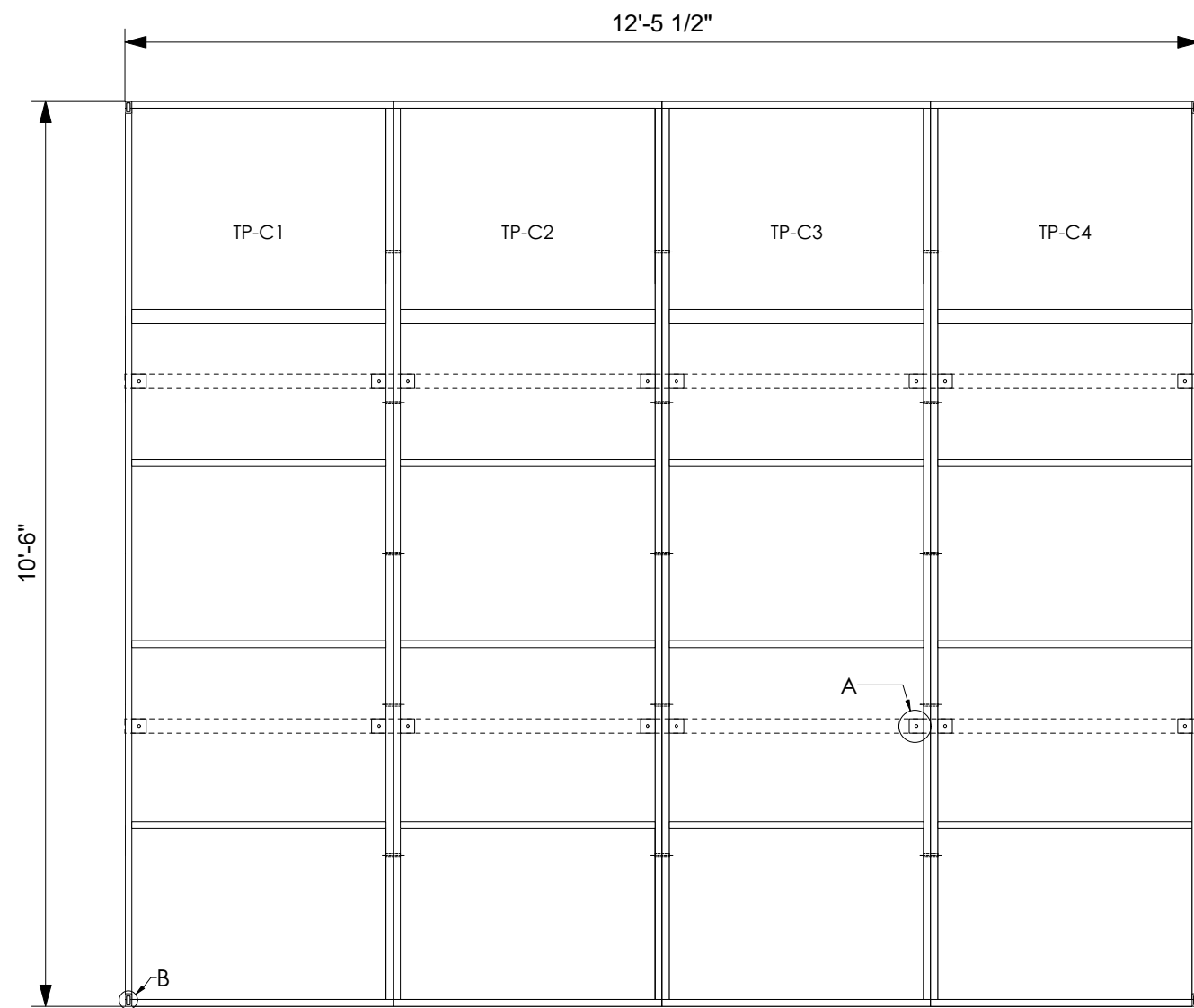
Ceiling Top View See Next Plate for Construction Information
