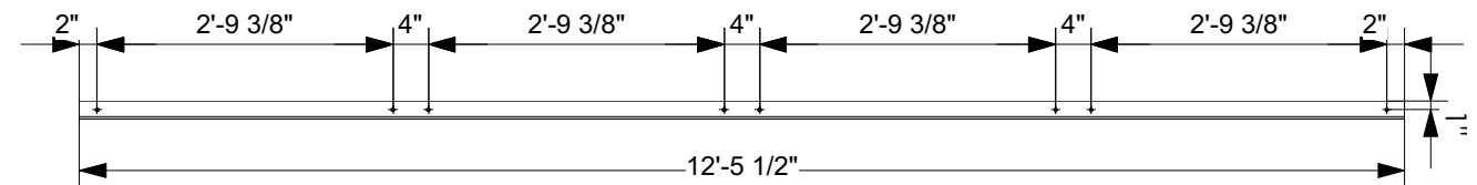
Ceiling Supports 2x2 Angle Drill 7/16\"/>
